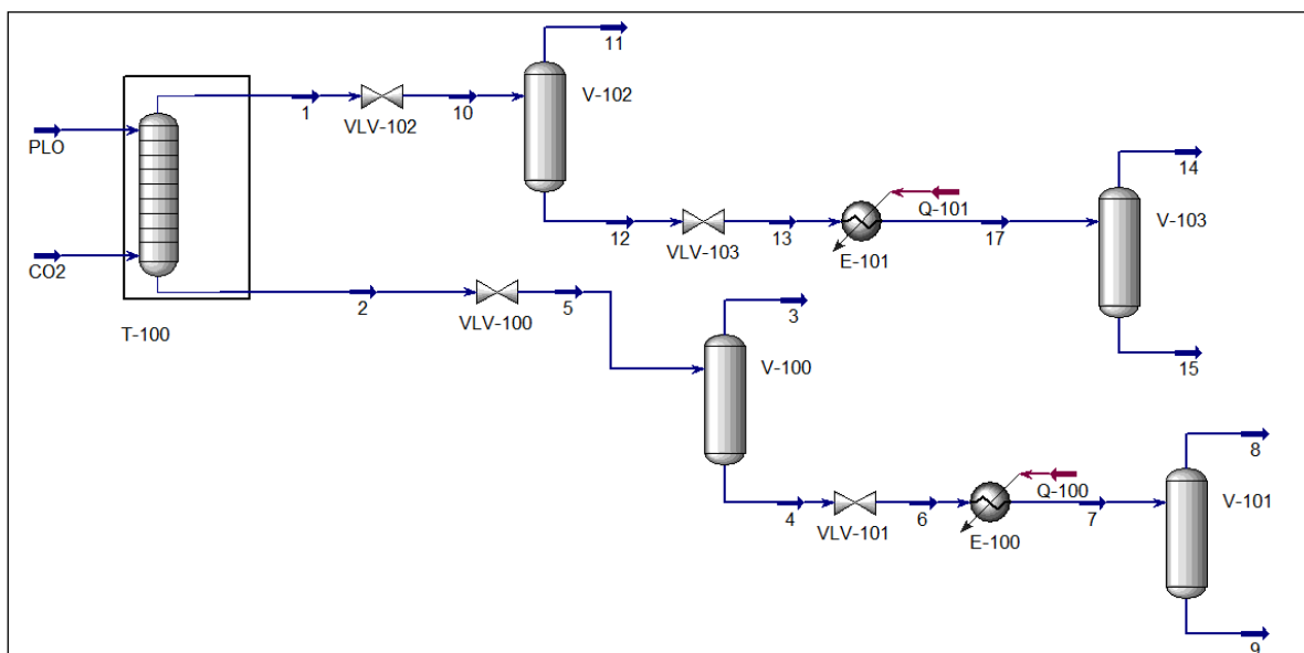
Figure 5.1 – Flowsheet 1 for OLP SFF.
