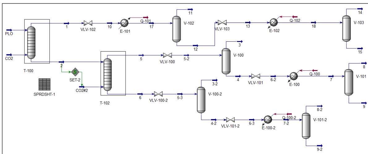
Figure 5.2 – Flowsheet 2 for OLP SFF (RAF1+ CO 2 as feed top stream and CO 2 make up as feed bottom stream),
