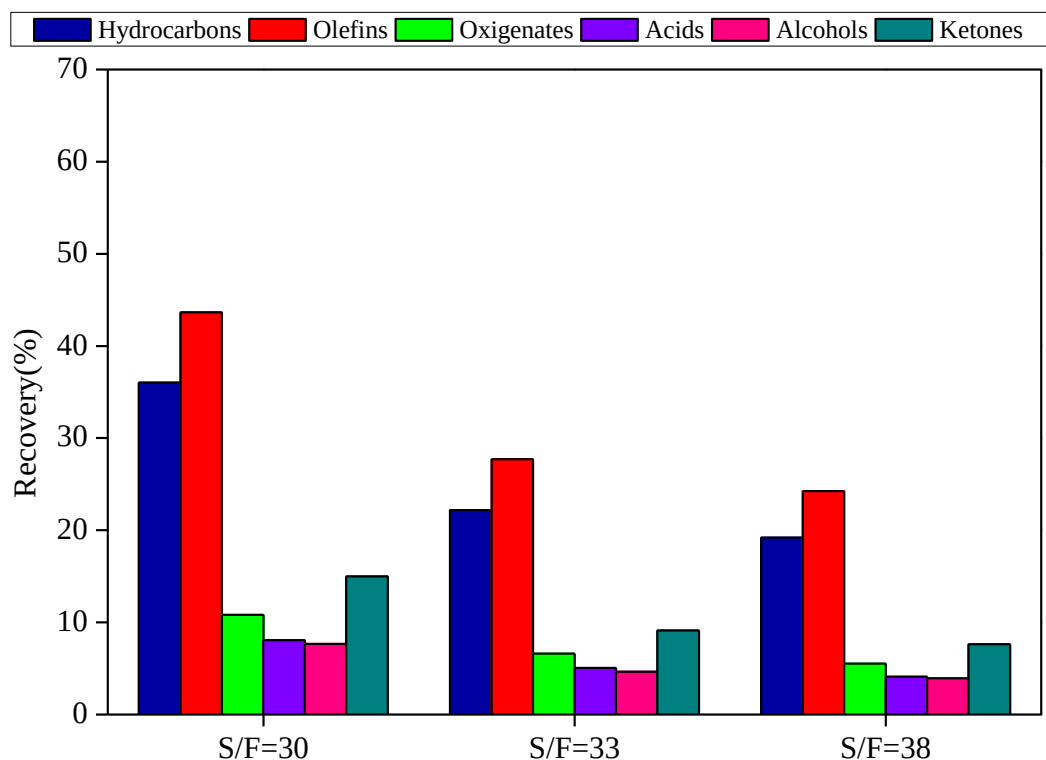
Figure 5.15 – Recovery of OLP fractions of SFF simulation in the top of column 2 (Flowsheet 3- column 1, S/F=17 ratio).
