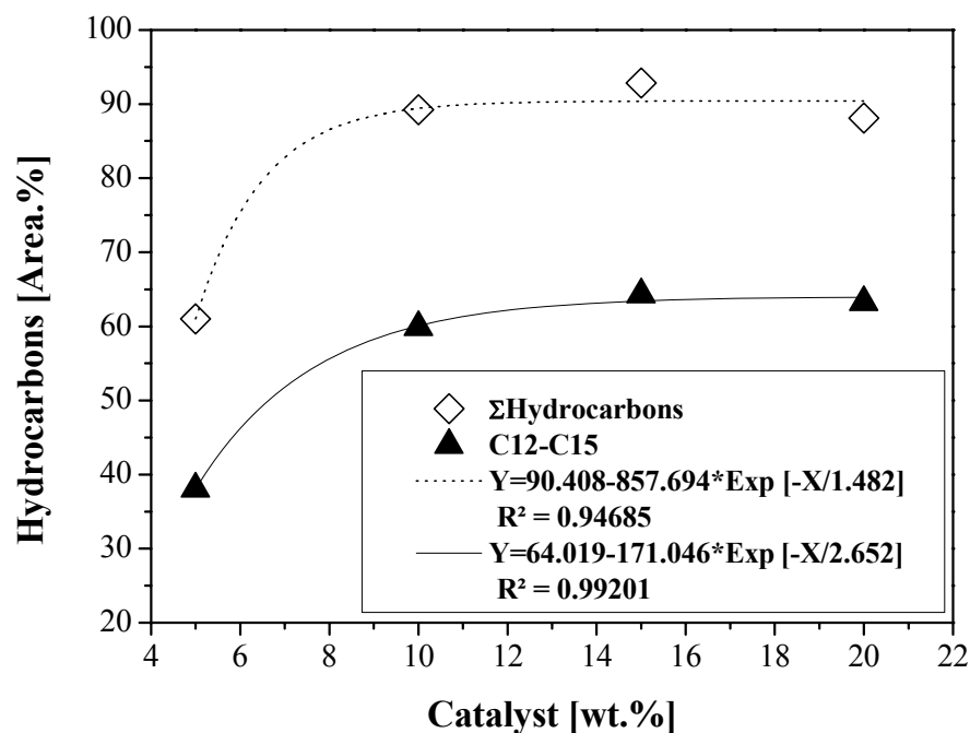
Figure 3. 11 - Summation of hydrocarbons and C12-C15 fractions present in OLP as a function of catalyst content.
