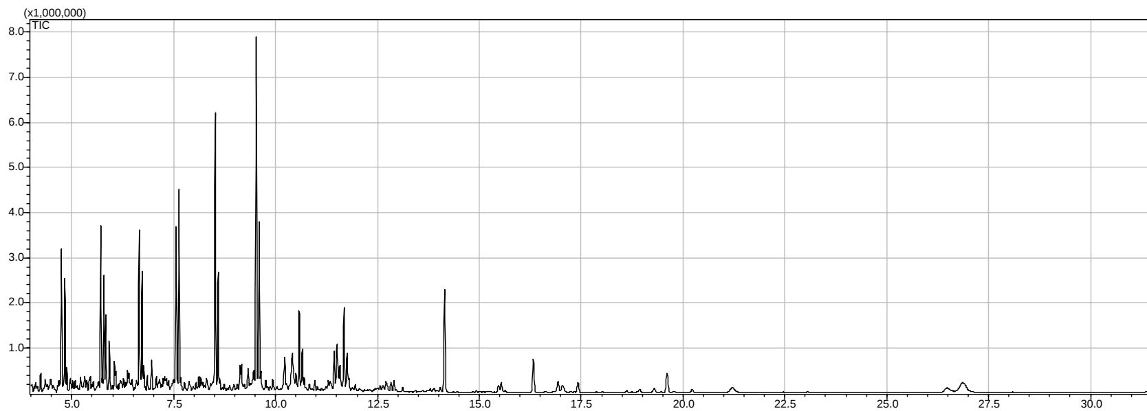
Figure A. 2 - CG-MS of OLP obtained by thermal catalytic cracking of palm oil with 10% (wt.) Sodium Carbonate at 450°C and 1 atm.
