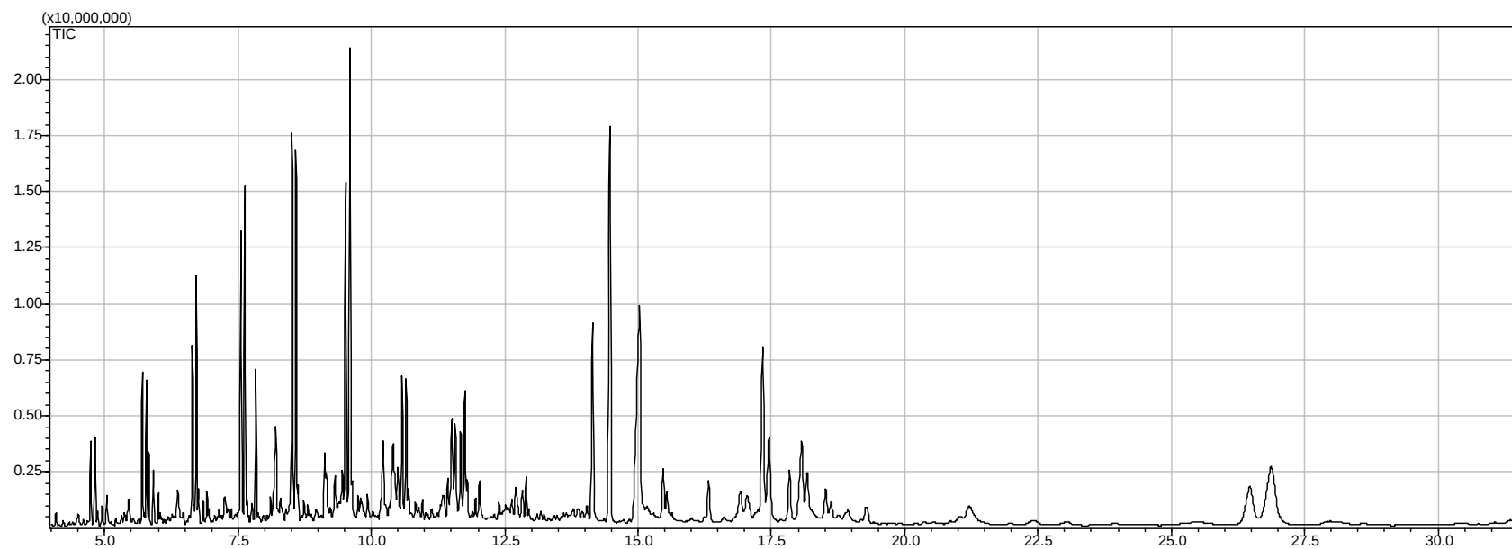
Figure A. 1 - CG-MS of OLP obtained by thermal catalytic cracking of palm oil with 5% (wt.) Sodium Carbonate at 450°C and 1 atm.
