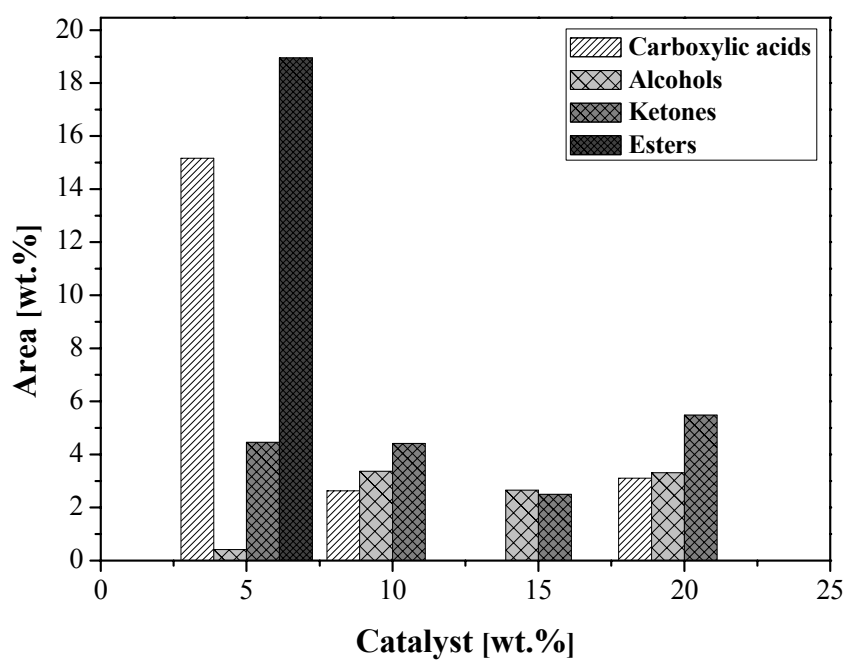
Figure 3. 14 – Distribution of oxygenated compounds present in OLP as a function of catalyst content.
