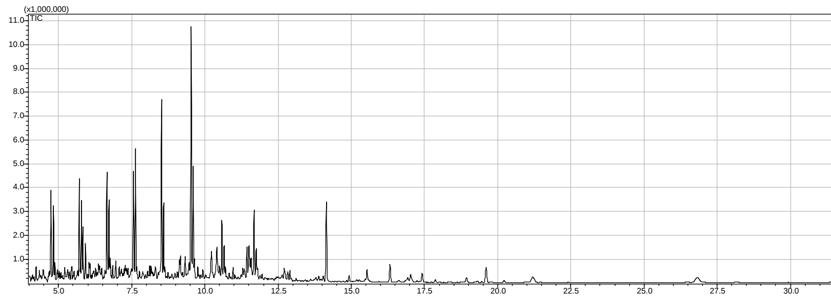
Figure A. 4 - CG-MS of OLIP obtained by thermal catalytic cracking of palm oil with 20% (wt.) Sodium Carbonate at 450°C and 1 atm.
