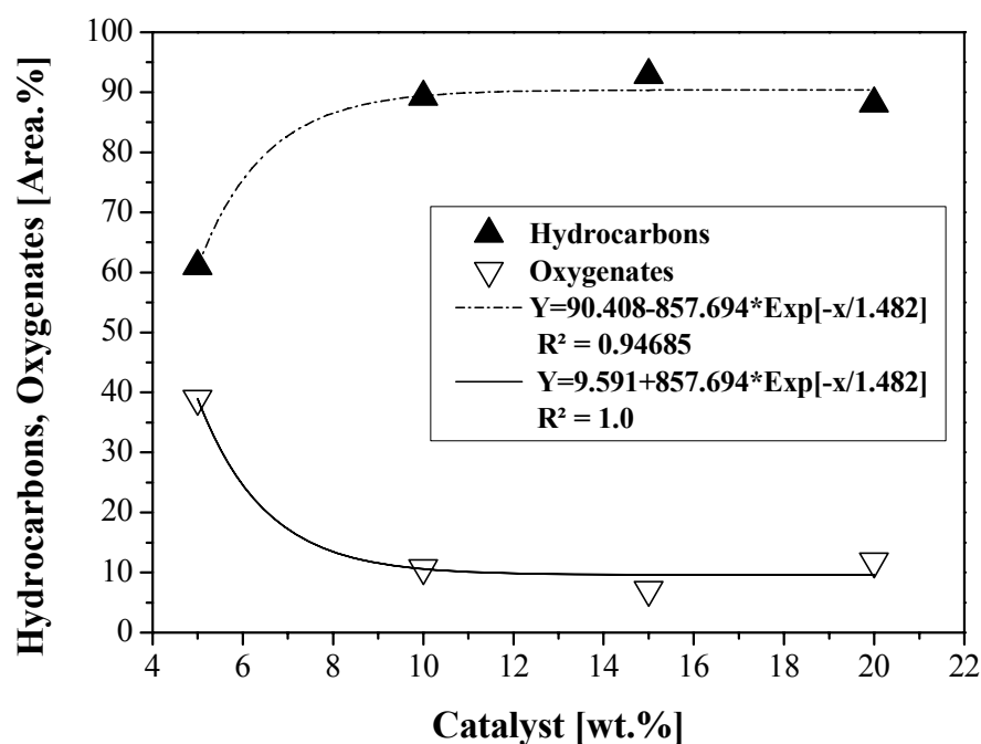
Figure 3. 10 - Distribution of hydrocarbons and oxygenated compounds presents in OLP as a function of catalyst content.
