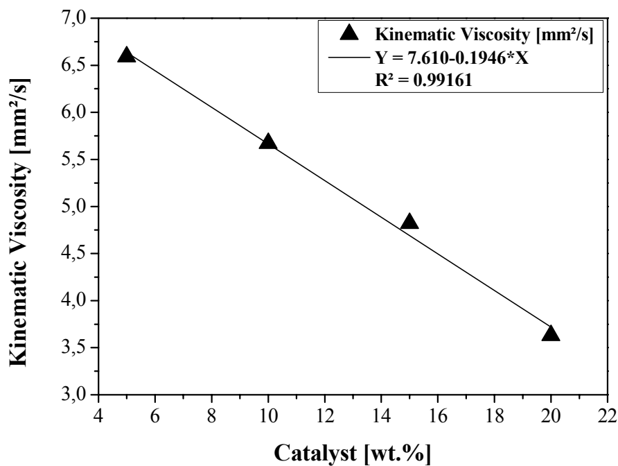
Figure 3. 8 - Kinematic Viscosity of OLP as a function of catalyst content.
