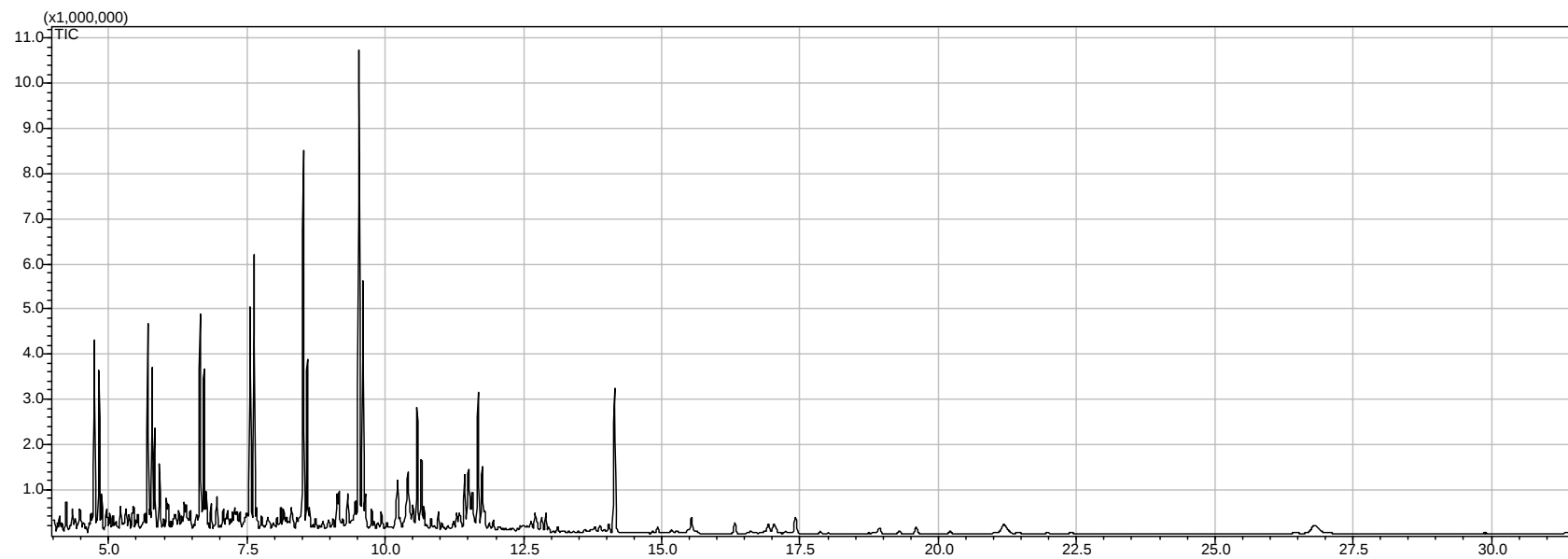
Figure A. 3 - CG-MS of OLIP obtained by thermal catalytic cracking of palm oil with 15% (wt.) Sodium Carbonate at 450°C and 1 atm.
