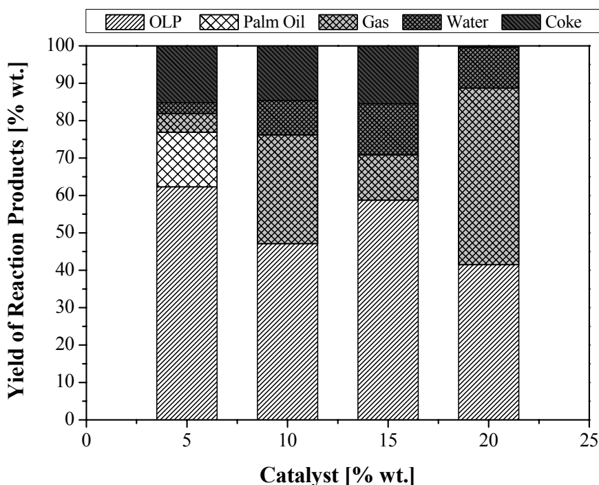
Figure 3. 6 - Yield of reaction products for the thermal catalytic cracking of palm oil at 450°C and 1 atm as a function of catalyst ( \text{Na}_2\text{CO}_3 ) content.
